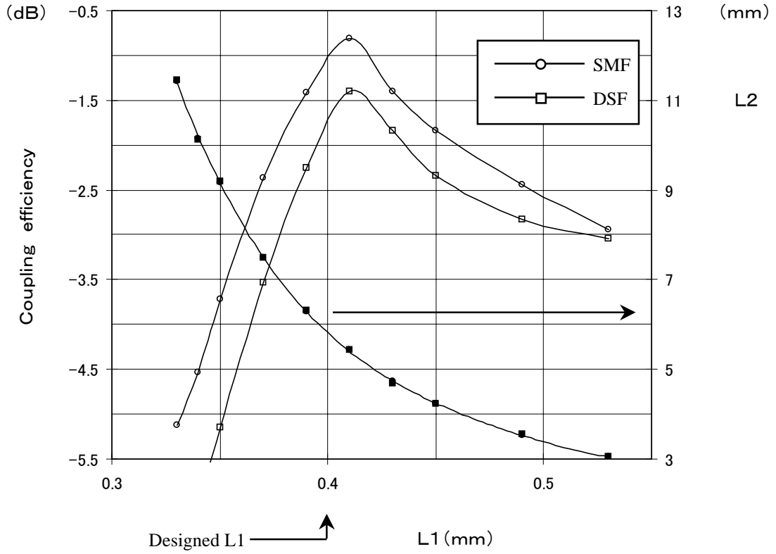
L2 and Coupling efficiency VS. L1
