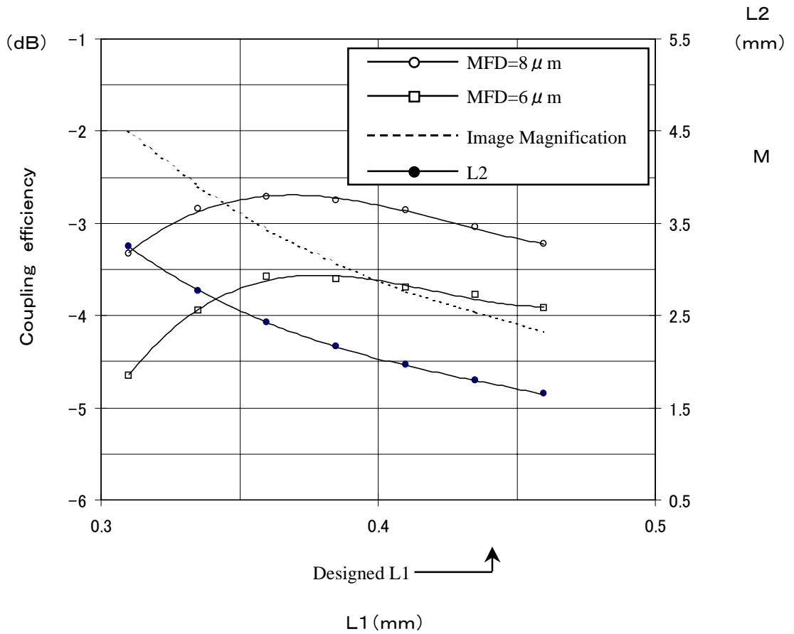
L2 and Coupling efficiency VS. L1
