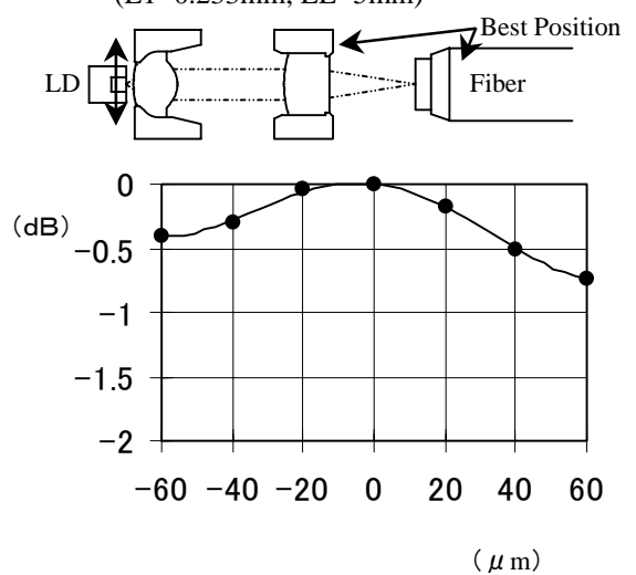
Excess Loss VS. 2nd Lens Block displacement (L1=0.233mm, LL=5mm)
