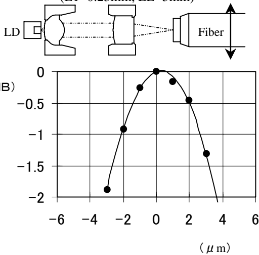
Excess Loss VS. 2nd Lens Block displacement (L1=0.23mm, LL=5mm)
