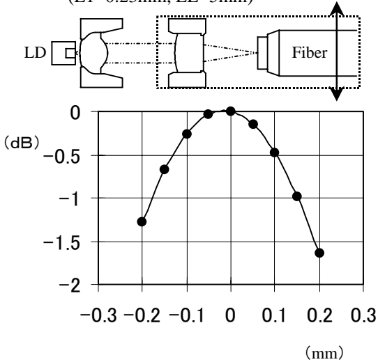
Excess Loss VS. 2nd Lens Block displacement (L1=0.23mm, LL=5mm)
