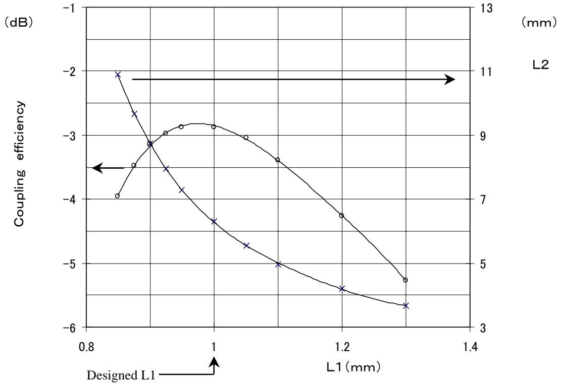
L2 and Coupling efficiency VS. L1
