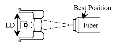
LD X tolerance
