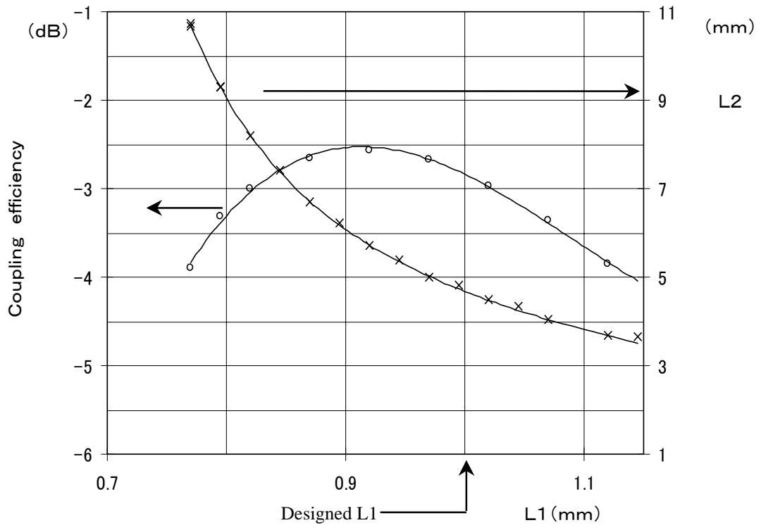
L2 and Coupling efficiency VS. L1
