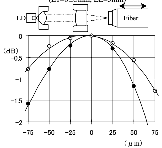
Excess Loss VS. Fiber Z displacement (L1=0.33mm, LL=5mm)
