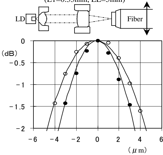
Excess Loss VS. Fiber X displacement (L1=0.33mm, LL=5mm)
