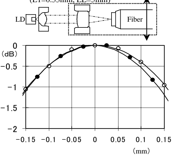
Excess Loss VS. 2nd Lens Block displacement (L1=0.33mm, LL=5mm)
