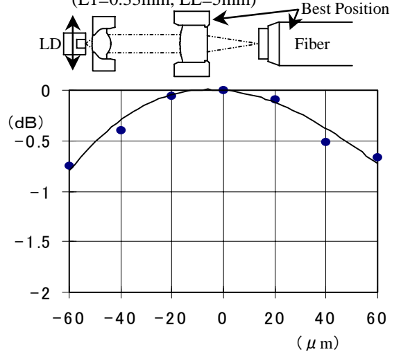
Excess Loss VS. 2nd Lens Block displacement (L1=0.33mm, LL=5mm)
