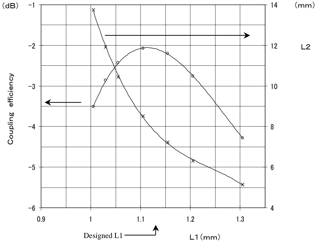
Fiber X tolerance
